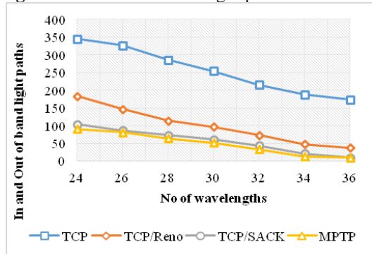
Fig. 8: In- and out-of-band light paths of COST239
