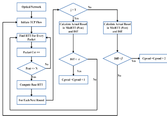
Fig. 3: Flow of the proposed TCP Vegas
