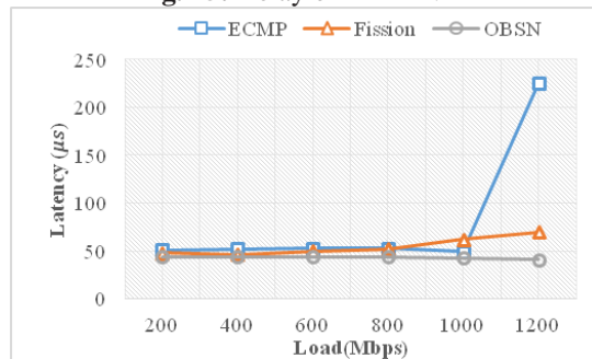
Fig. 16: Latency
