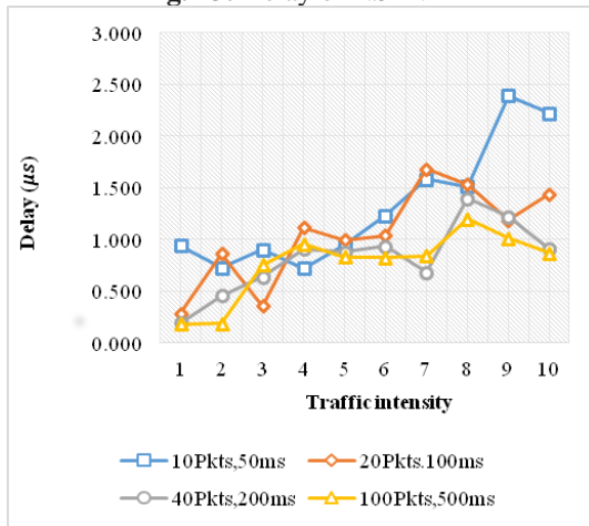
Fig. 14: Delay of COST239
