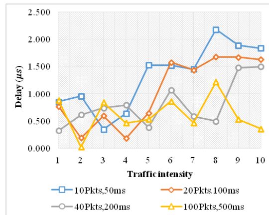
Fig. 15: Delay of ARPANET
