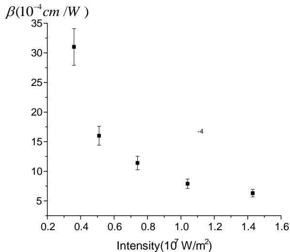
Fig . 5. Variation of nonlinear absorption coefficient \beta at \lambda=633 nm as a function of input intensity
