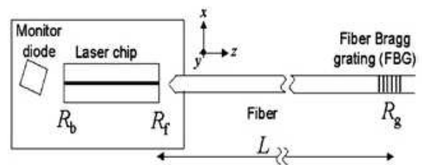
Fig. 8: Schematic of an FBG-stabilized pump laser module. R_b , R_f , and R_g denote the back, front, and FBG power reflectivity[29]
