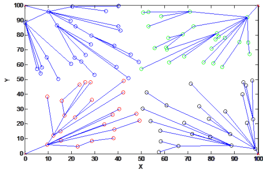
Figure 2: Partition site and make shortest path from each node to a sink
