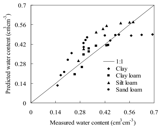
Fig. 4 Comparison of predicted water content of Rosetta with that of measurement [21] ( R^2 = 0.585 ).
