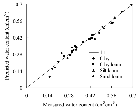
Fig. 3 Comparison of the predicted water content of RETC with that of measurement [21] ( R^2 = 0.974 ).
