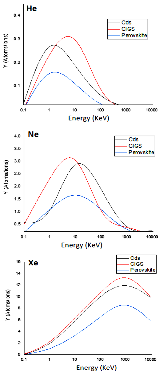
Figure 1: Sputtering yield as a function of energy for photovoltaic cells of Cds, CIGS, and Perovskite materials bombarded by (a) Argon, (b) helium, (c) Neon, (d) Xenon gases
