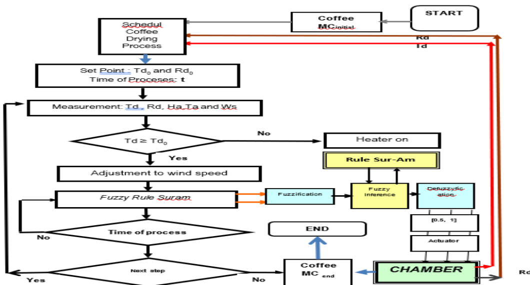
Fig. 12: Block Diagram of Fuzzy Rule
