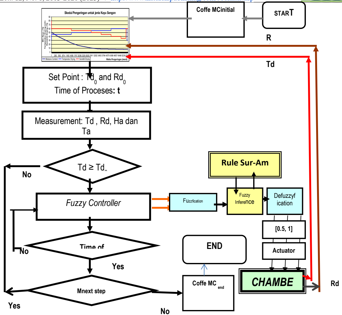
Fig. 9: Block Diagram of Intelligent Fuzzy Controller
