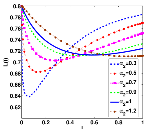
L(t) for \alpha_1 = 0.3, \alpha_3 = 0.9
