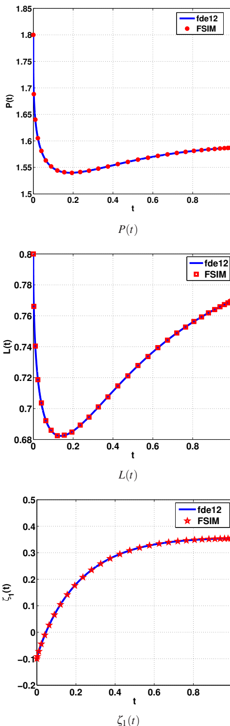
Fig. 2: plot of the variables P, L, \zeta_1 for T = 1, N = 32 collocation points and h = 10^{-5} for the fde12 method
