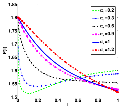
P(t) for \alpha_2 = 0.5, \alpha_3 = 0.9
