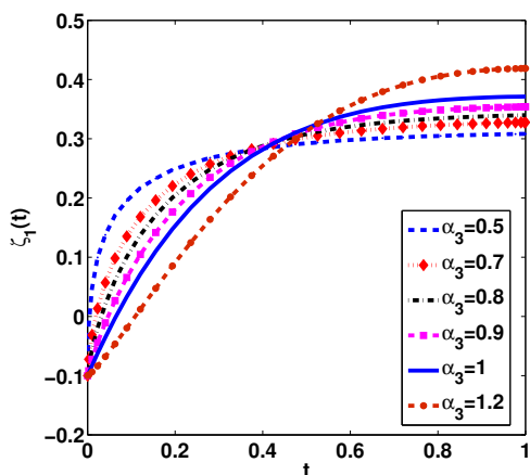
\zeta_1(t) for \alpha_2 = 0.3, \alpha_2 = 0.5
