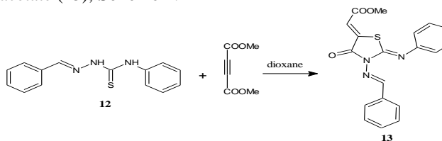
Scheme 4: Reaction of benzylidene-carbothioamide 12 with DMAD in dioxane.
