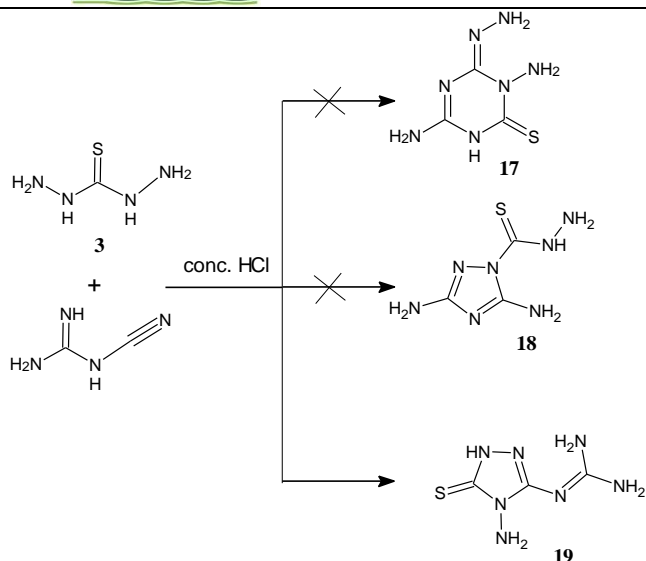
Scheme 7: Reaction of thiocarbohydrazide 3 with CG in concentrated HCl
