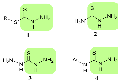
Fig. 2: Reagents containing carbothiohydrazides
