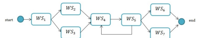
Figure 1. Service composition workflow
