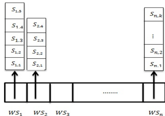
Figure 4. Genetic Encoding scheme.
