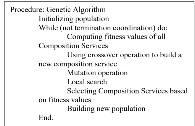
Figure 3. A hybrid genetic algorithm for the online business service selection problem
