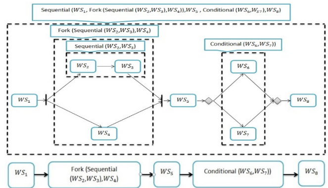
Figure 1. Aggregation process example of QoS properties.
