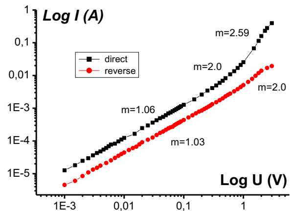
Fig. 5: Dark I-V characteristic of the n-SnO 2 /p-Si photoelectric heterojunction constructed on a double logarithm scale
