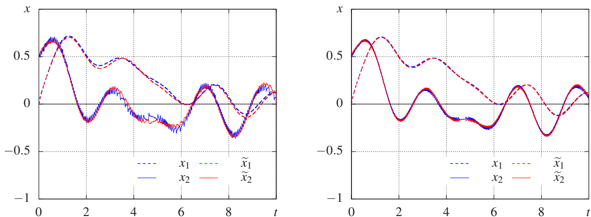
Fig. 2: The realized motions x(\cdot) of system (41), (42) and their approximations \tilde{x}(\cdot) for h = 0.1 , \delta = 0.02 and h = 0.01 , \delta = 0.005 .
