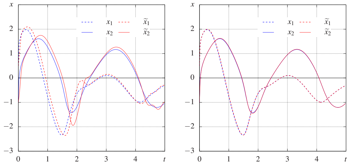
Fig. 1: The obtained solution x(\cdot) of Cauchy problem (24), (25) and its approximations \tilde{x}(\cdot) for h = 0.1 and h = 0.01 .
