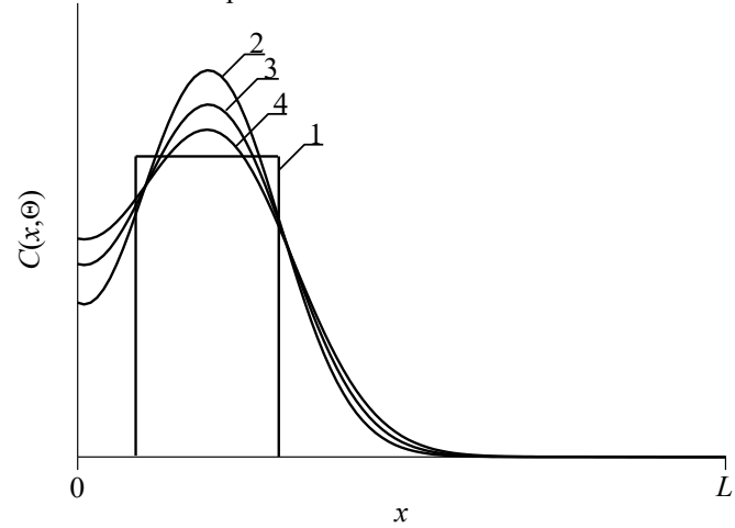
Fig. 5: Spatial distributions of dopant in heterostructure after ion implantation. Curve 1 is idealized distribution of dopant. Curves 2-4 are real distributions of dopant for different values of annealing time. Increasing of number of curve corresponds to increasing of annealing time.
