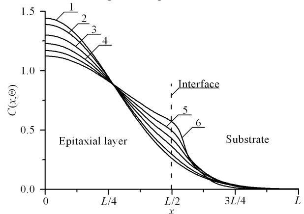
Fig. 2: Distributions of concentration of infused dopant in heterostructure from Fig. 1 in direction, which is perpendicular to interface between epitaxial layer substrate. Increasing of number of curve corresponds to increasing of difference between values of dopant diffusion coefficient in layers of heterostructure under condition, when value of dopant diffusion coefficient in epitaxial layer is larger, than value of dopant diffusion coefficient in substrate.
