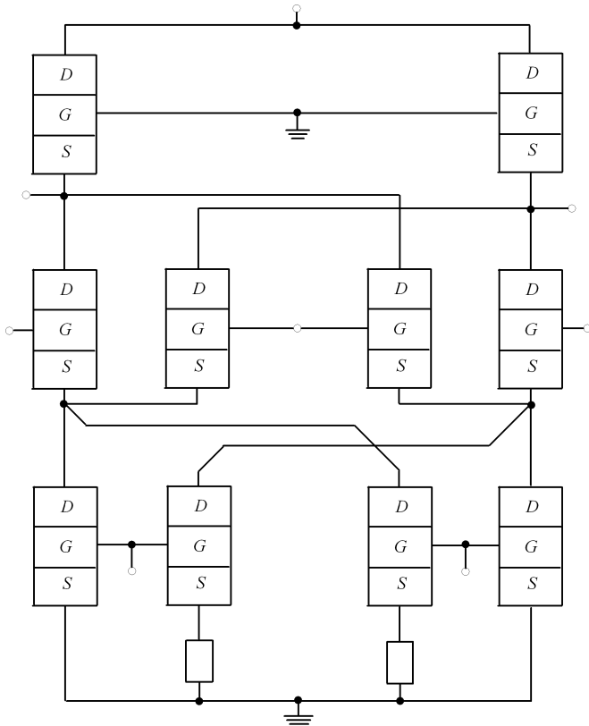
Fig. 1a: Structure of the considered circuits.
