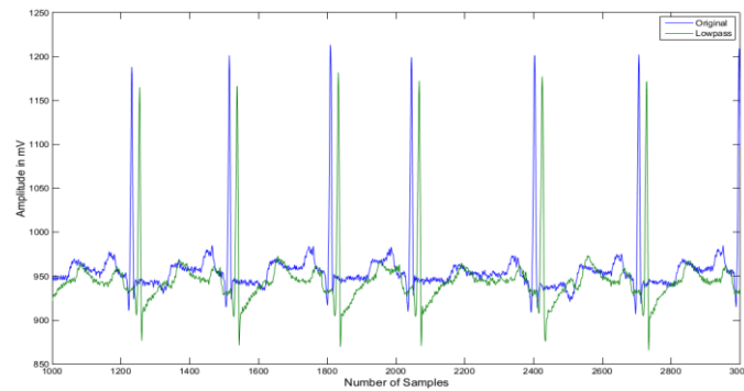
Figure 18. Chebyshev-II Filtered Signal
