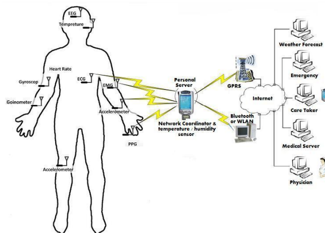
Figure 1. Wireless Body Area Network Scheme
