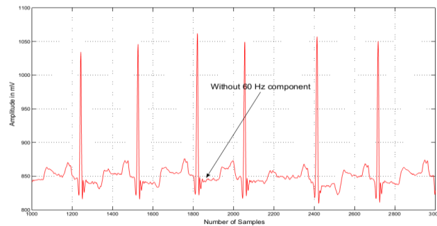
Figure 25. 60 Hz Notch Filter
