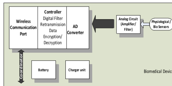
Figure 3. Functional Block Diagram
