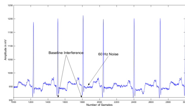
Figure 6. Original Signal with Noise
