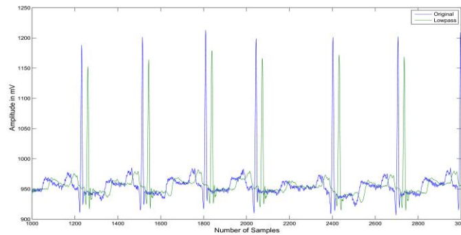
Figure 17. Chebyshev-I Filtered Signal
