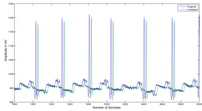
Figure 22. Hamming Window based Filtered Signal
