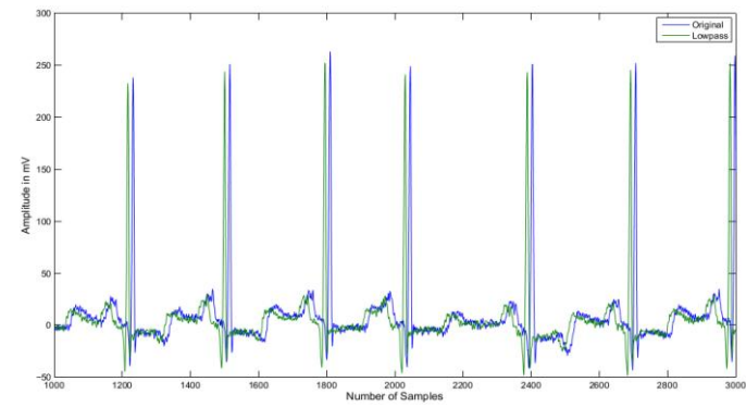
Figure 24. Blackman Window based Filtered Signal
