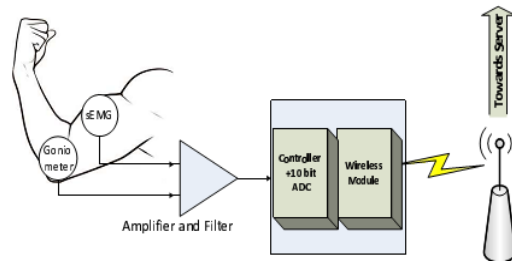
Figure 4. Overview of Hardware Architecture
