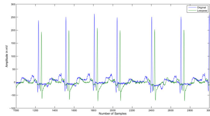
Figure 19. Elliptical Lowpass Filtered Signal
