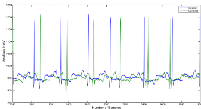
Figure 21. Hanning Window based Filtered Signal
