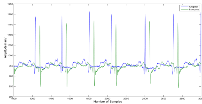
Figure 16. Butterworth Filtered Signal
