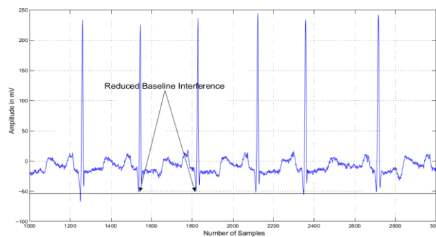
Figure 11. Kaiser Window based Highpass Filter
