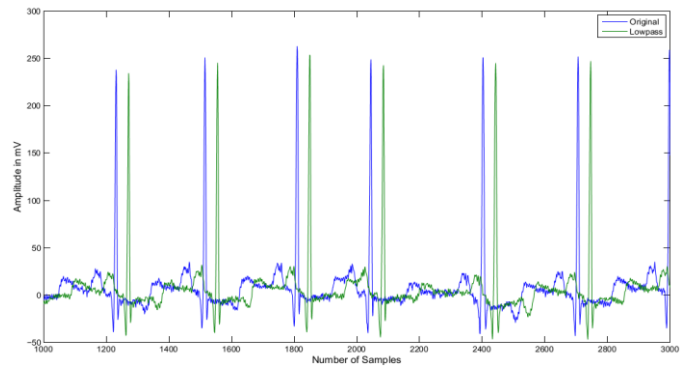
Figure 23. Blackman Window based Filtered Signal
