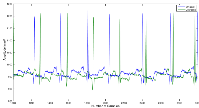
Figure 20. Kaiser Window based Filtered Signal
