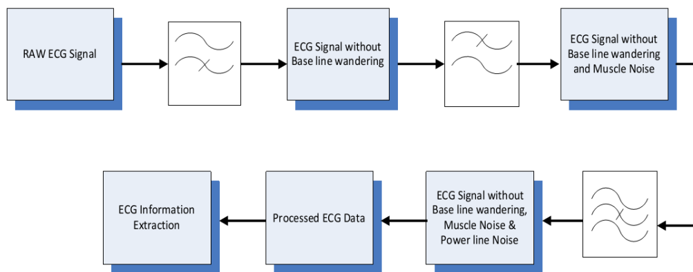
Figure 5. ECG Signal Processing Flow Diagram
