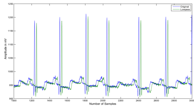
Figure 22. Hamming Window based Filtered Signal
