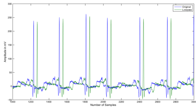
Figure 23. Blackman Window based Filtered Signal
