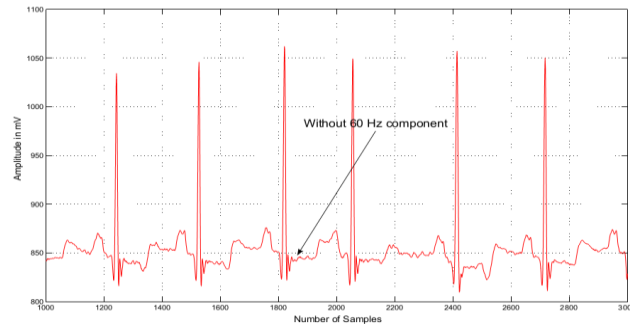
Figure 25. 60 Hz Notch Filter
