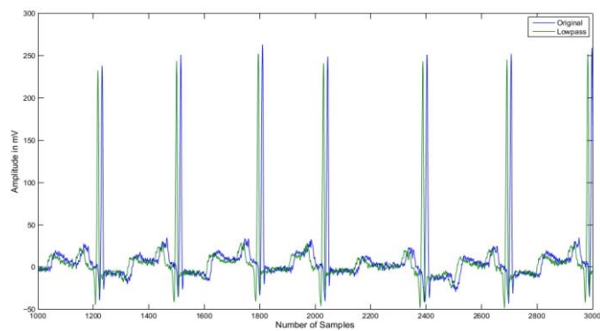
Figure 24. Blackman Window based Filtered Signal
