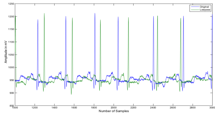
Figure 21. Hanning Window based Filtered Signal
