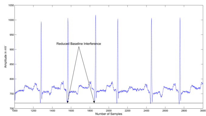
Figure 15. Blackman Harris Window based Highpass Filter
